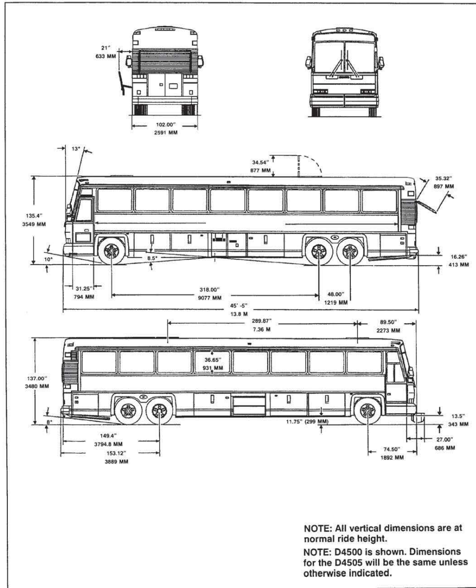
Figure 3. D4500 Model Body and Door Clearance Diagram
